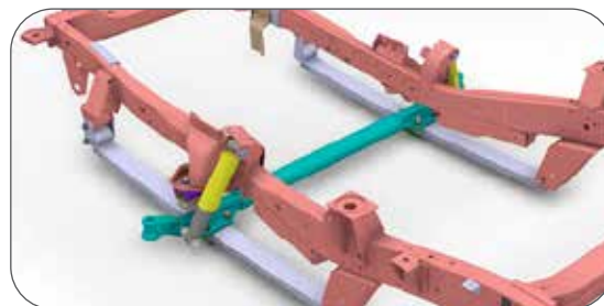
DURABLE RIGID FRONT LEAF SPRING SUSPENSION
